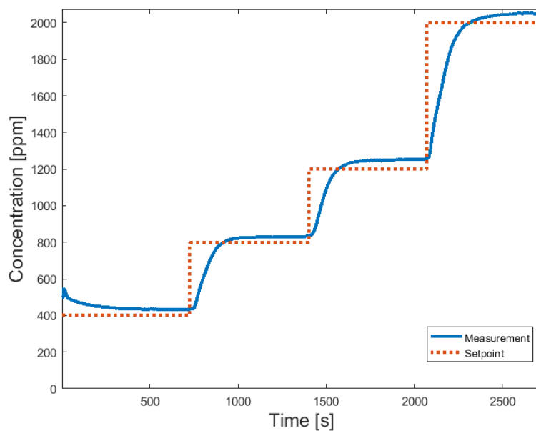
Fig. 6. MHZ19C response to different CO 2 concentrations.
