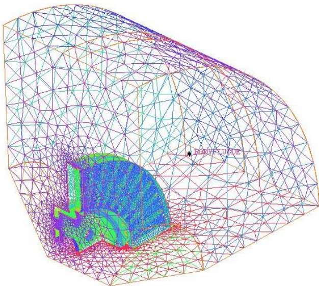
Figure 13. Meshing for a fluid body.
