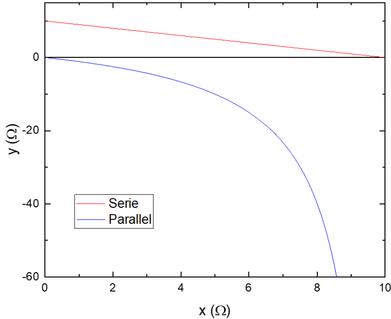
Figure 2. Resistance 2 ( \equiv y ) as a function of resistance 1 ( \equiv x ) with R_{eq} = 10\Omega
