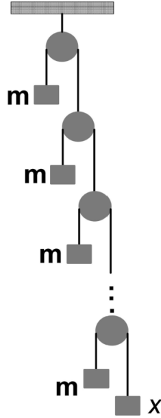
Figure 1. An Atwood machine composed of n identical masses m connected in series, together with an additional mass x attached to the final pulley
