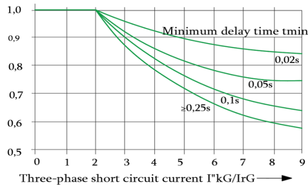
Figure 5. Factor \mu for calculating short-circuit breaker current
