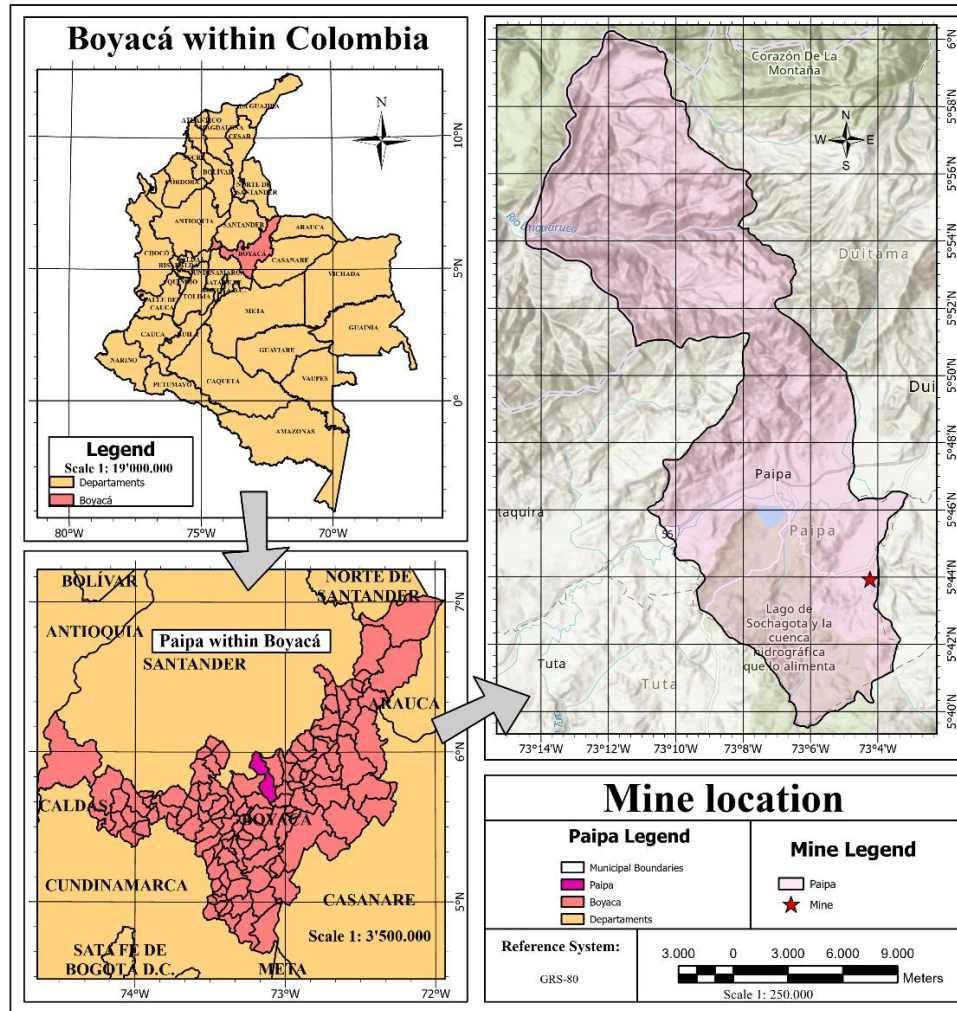
Figure 1. Location of the municipality of Paipa, Colombia.
