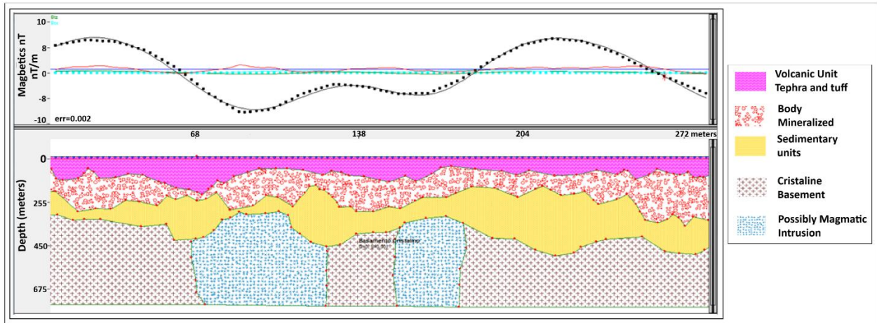
Figure 9. (a) Observed and calculated fields (solid black line: calculated field; dotted black line: observed field). (b) Geological–geophysical model, Profile 1.
