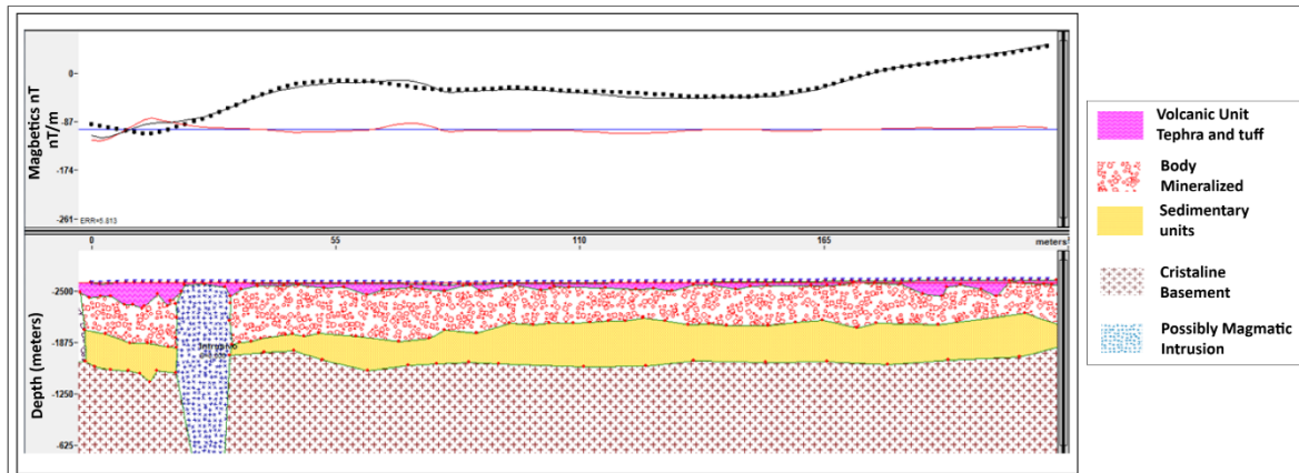
Figure 10. (a) Observed and calculated fields (solid black line: calculated field; dotted black line: observed field). (b) Geological–geophysical model, Profile 2.
