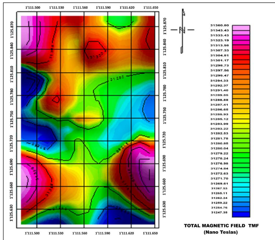
Figure 6. Total magnetic field map (TMF).
