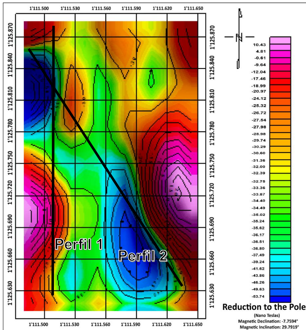
Figure 8. Map of anomalies with reduction to pole. Profiles drawn for 2D modeling are shown in black.
