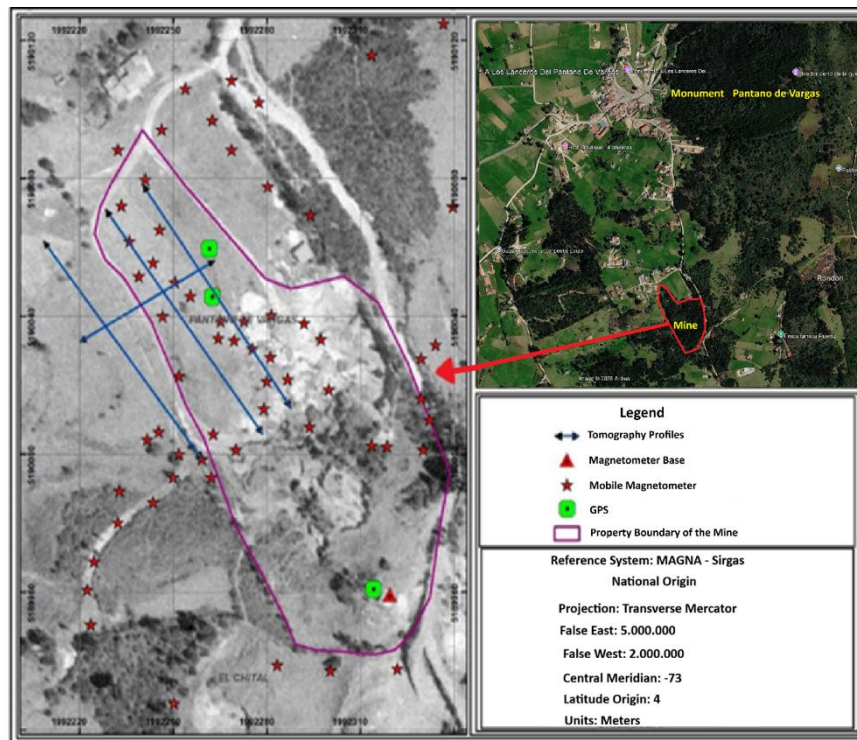
Figure 5. GPS location, magnetic sampling points and electrical profiles.
