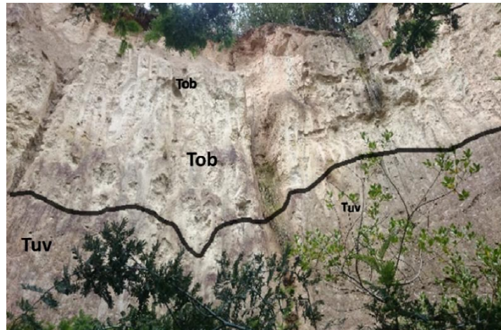
Figure 3. Segments 1 and 2 Tobas del Guarrús deposit (Tob), below the El Volador Tertiary Unit (Tuv).
