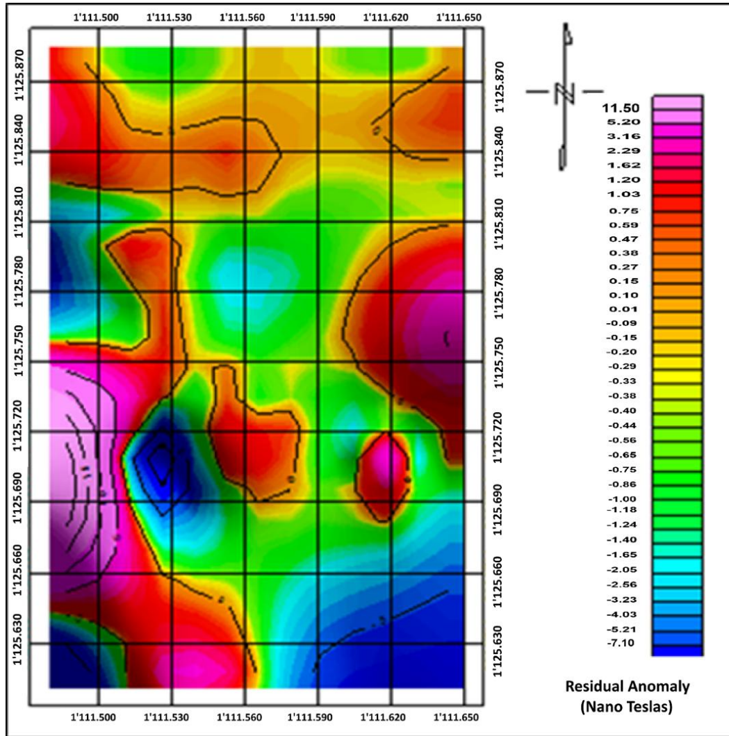
Figure 7. Map of residual anomalies (RA).
