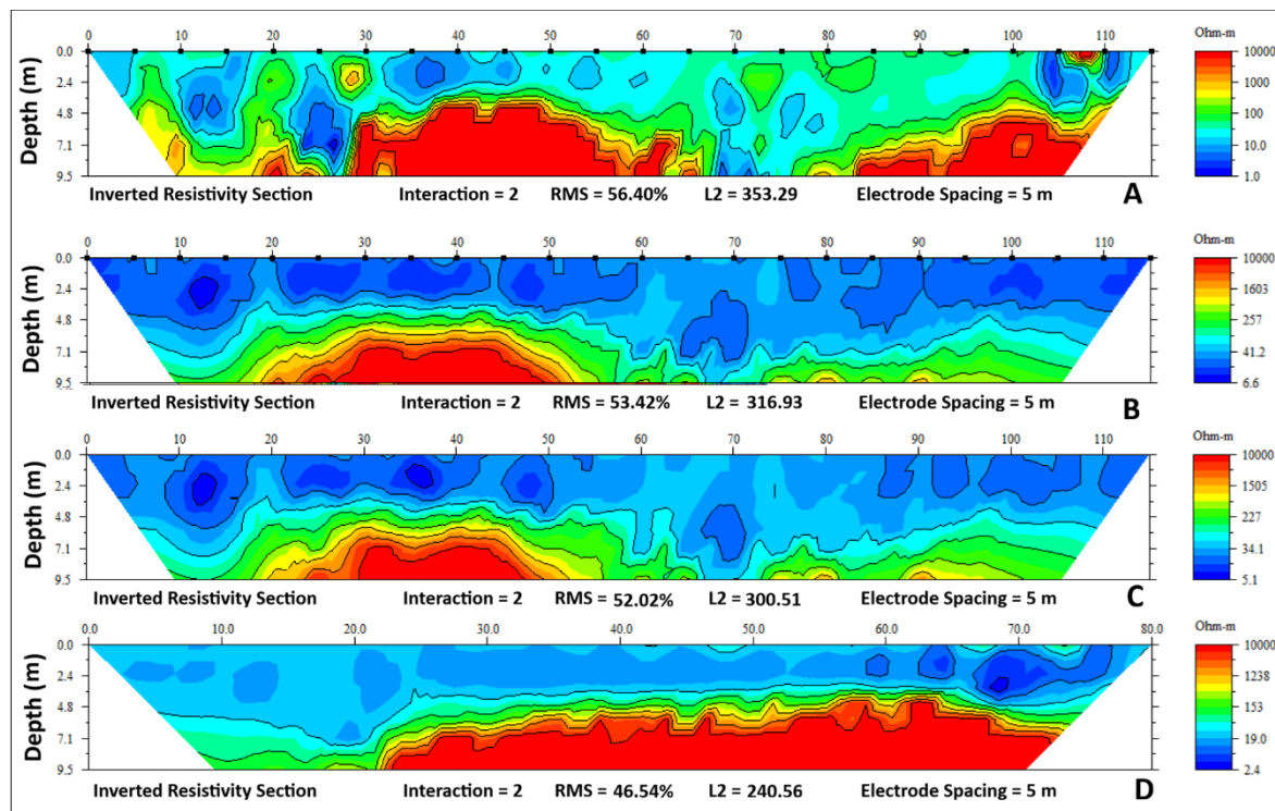
Figure 11. Resistivity tomography. True resistivity distribution: (a) Profile 1 (110 m), (b) Profile 2 (110 m), (c) Profile 3 (110 meters), (d) Profile 4 (transverse).
