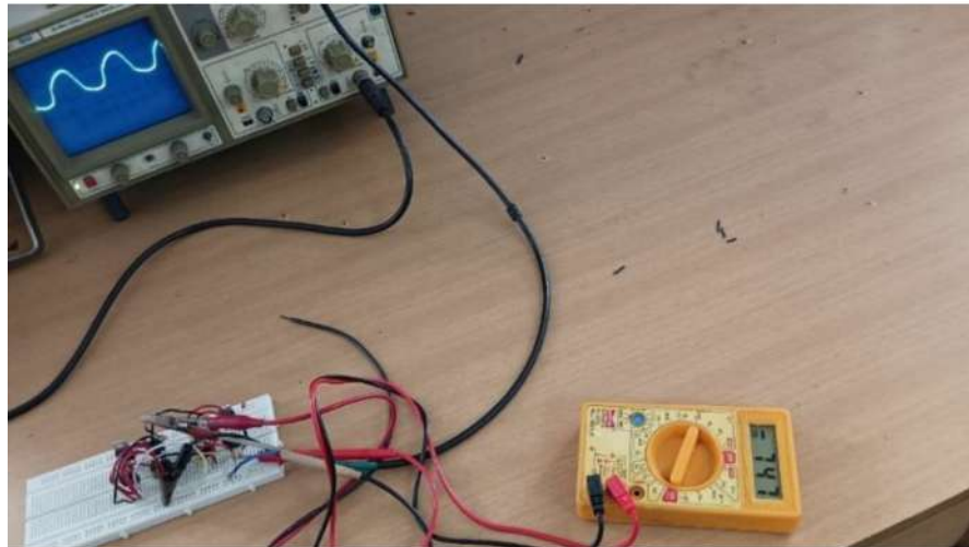
Figure 3. Rectified DC output voltage of the proposed circuit
