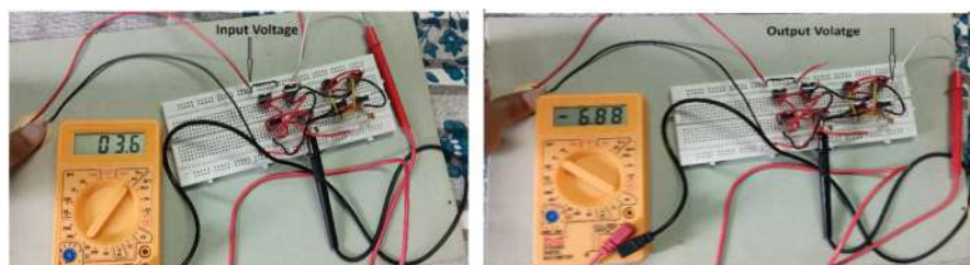
Figure 4. AC input and rectified DC output of the two-stage cross-coupled piezoelectric harvester
