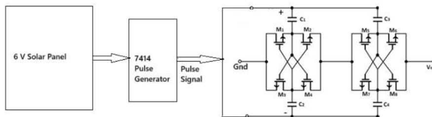
Figure 11. Solar-powered energy harvester
