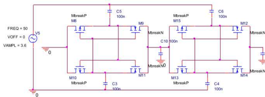
Figure 8. Two-stage cross-coupled MOS-based voltage multiplier circuit
