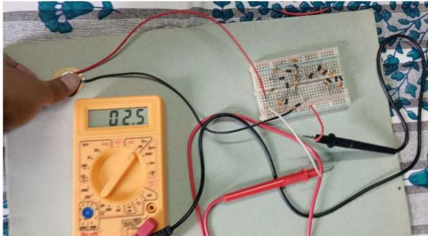
Figure 6. Input voltage from of the piezoelectric energy harvester with the diode-based circuit
