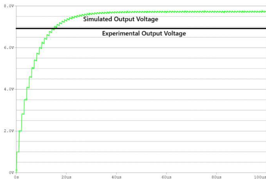
Figure 9. Comparison between experimental and simulated results
