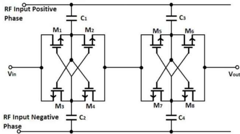
Figure 2. Two-stage cross-coupled MOS-based energy-harvesting circuit
