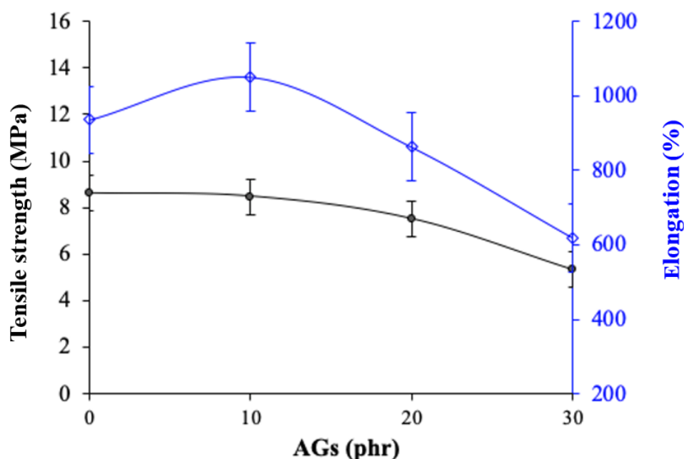
Figure 3. Tensile strength and elongation properties of NR/MDTAG
