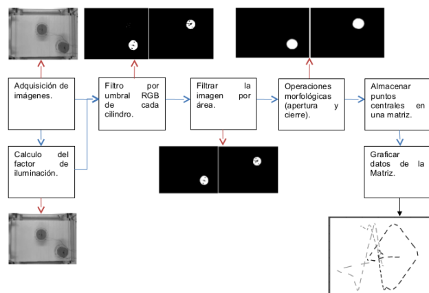
Figure 3: Flow diagram of image processing to obtain cylinders position.
