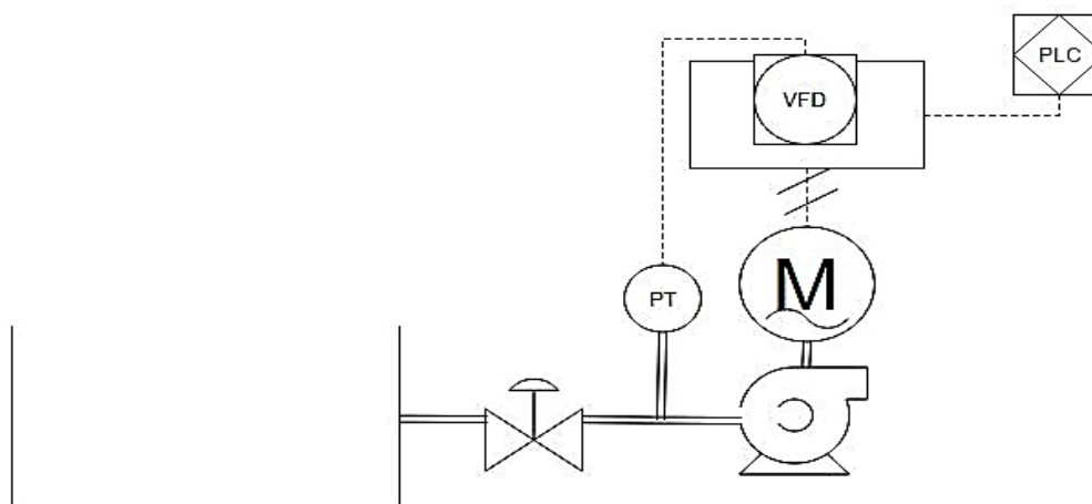
Figure 3. P&ID layout of system instruments.
