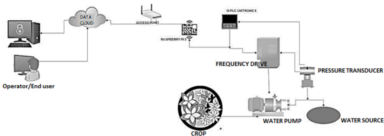
Figure 4. Basic structure of physical plant.
