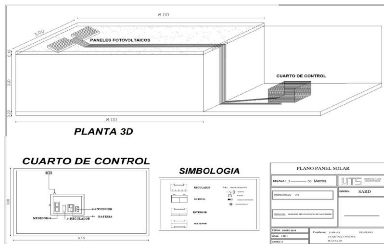
Figure 2 Prototype installation plan.
