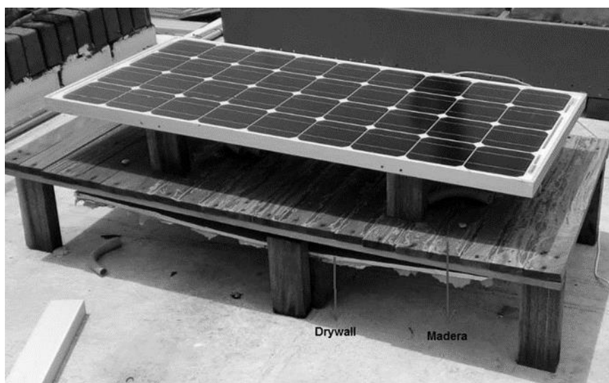
Figure 4. Wood and Drywall surface.
