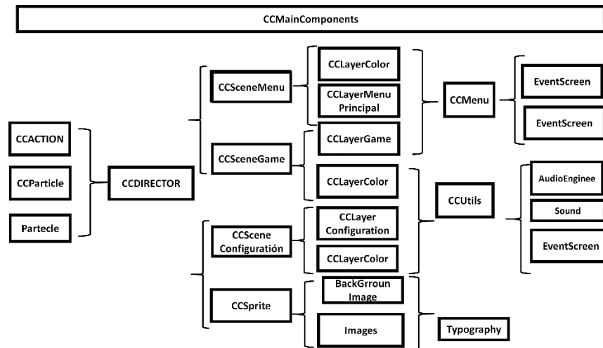
Figure 2: Architecture implemented in the labyrinth using Cocos2DX
