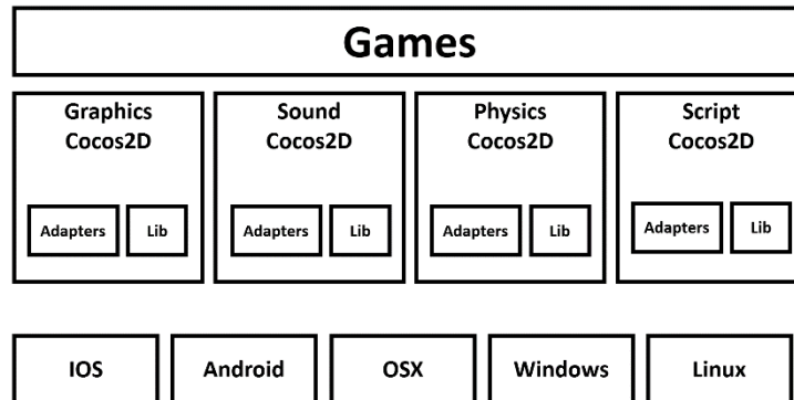
Figure 1: Based on [23] Cocos2DX Architecture
