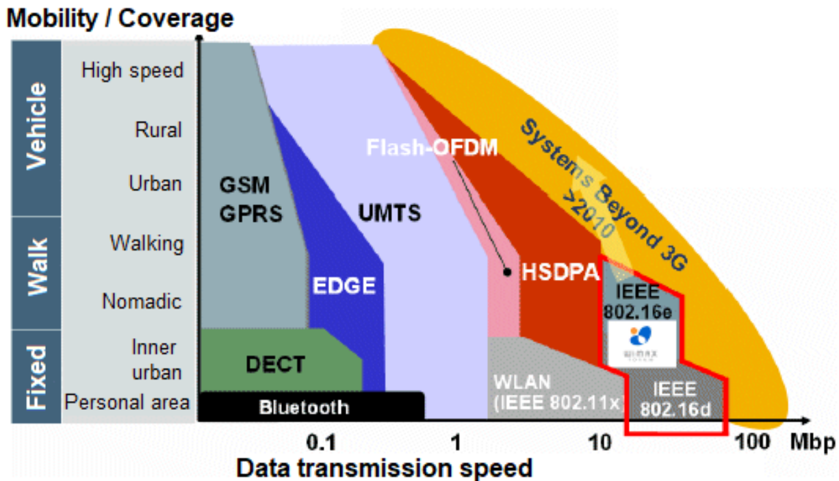
Figure 3. Transmission capacity and mobility of wireless technologies. [15]
