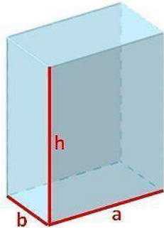
Figure 10. Volume of a right prism. [29]
