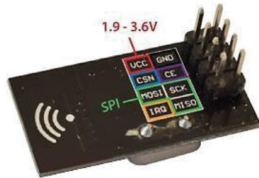
Figure 8. NRF24L01 pin configuration. [27]
