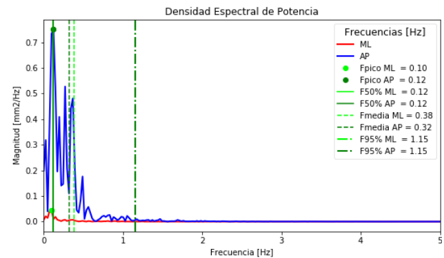
Figure 4. Frequency spectral density. [4].
