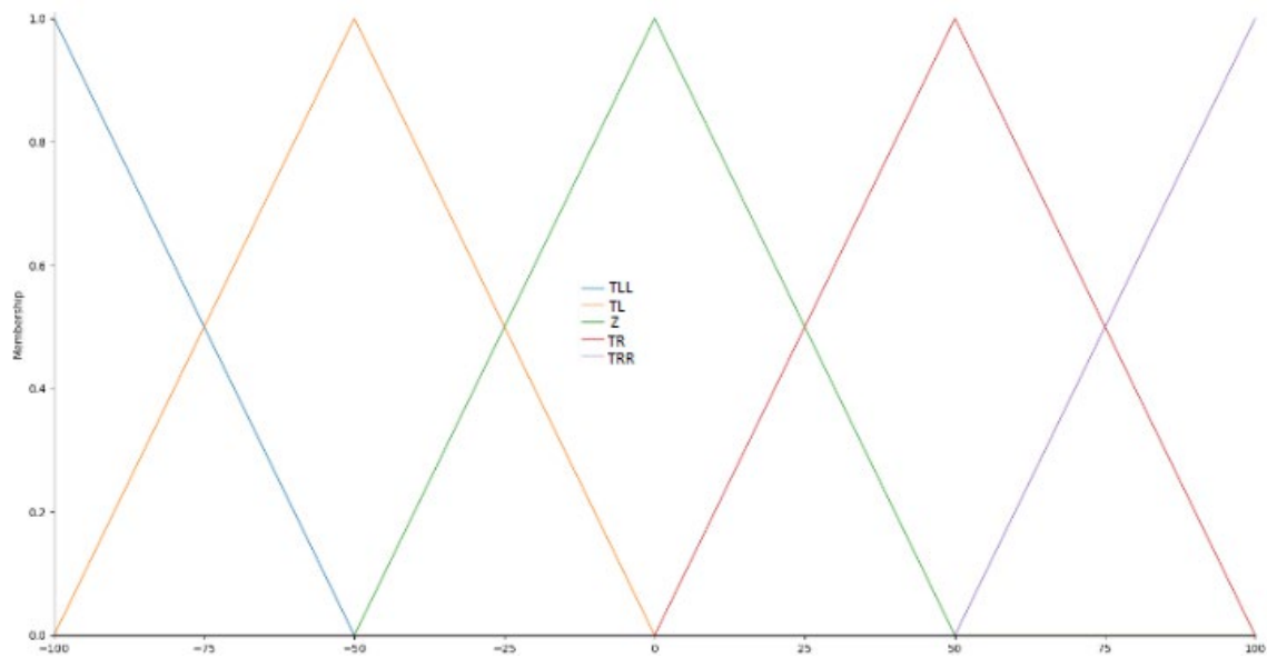
Figure 11. Output fuzzy sets.
