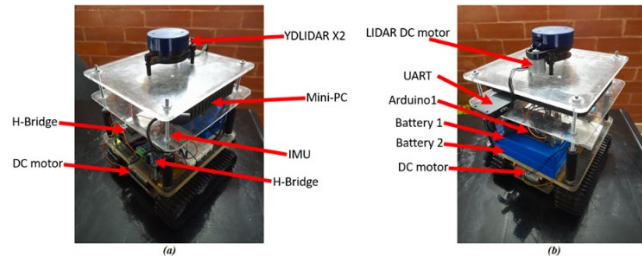
Figure 1. General view of Robot structure.
