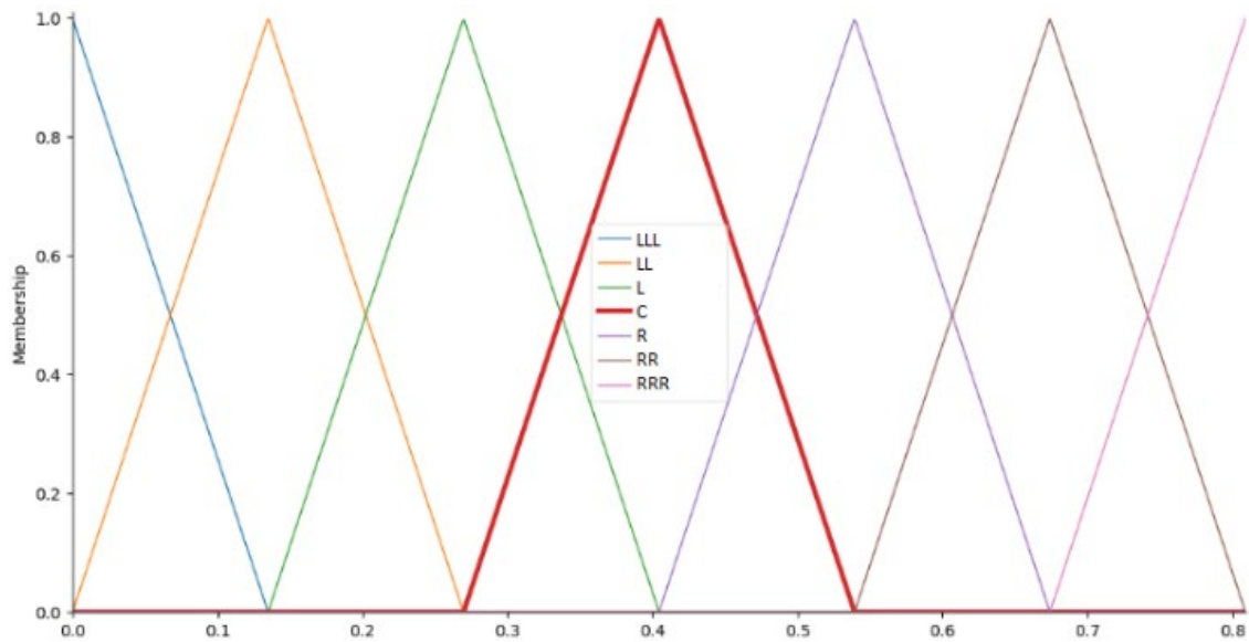
Figure 10. Input fuzzy sets.
