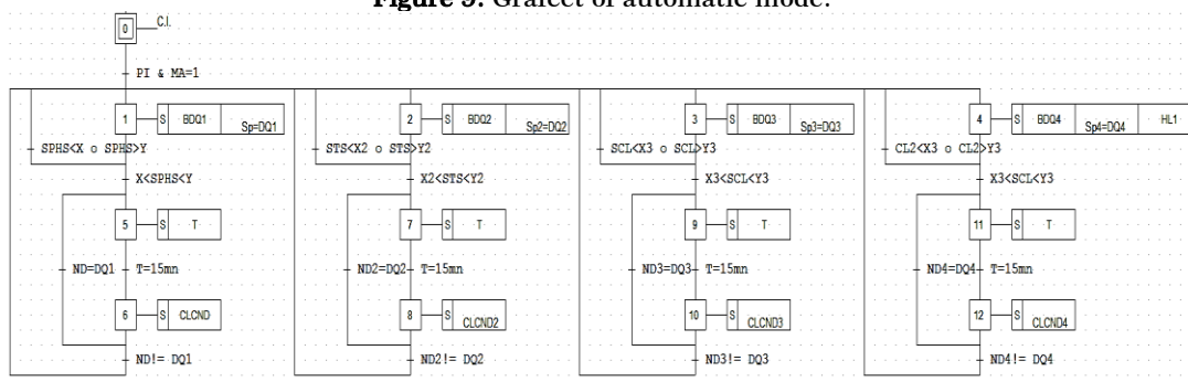
Figure 9. Grafcet of automatic mode.
