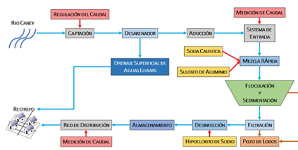
Figure 5. Emiliano Restrepo Echavarría DWTP process diagram.
