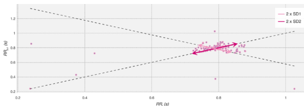
Figure 7. Poincare graph.
