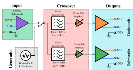
Figura 3: Two way active crossover.
