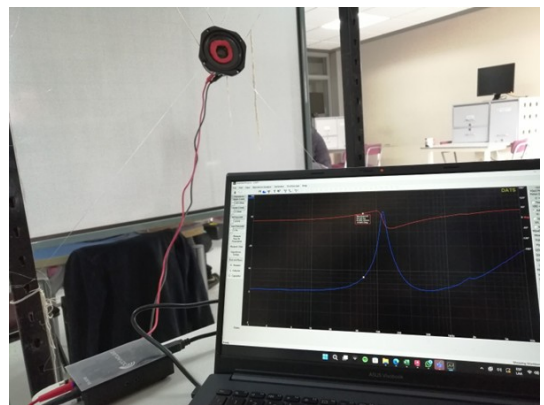
Figura 12: Impedance measurement with Mass using DATS V3
