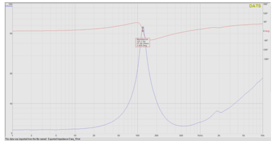
Figura 11: Impedance Response with DATS V3 method
