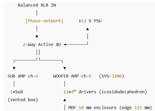
Figura 15: Connections of the electroacoustic subsystems
