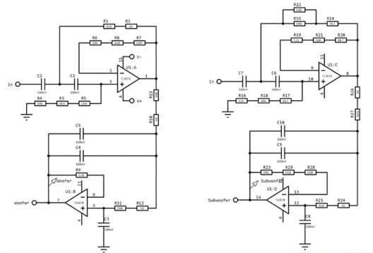
Figura 7: Filter for loudspeaker of a subwoofer type.
