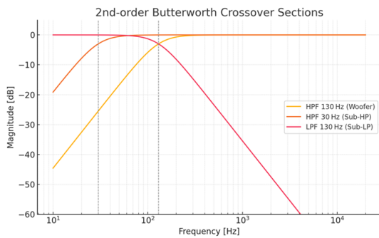
Figura 6: Frequency Response of implemented filters (Crossover)
