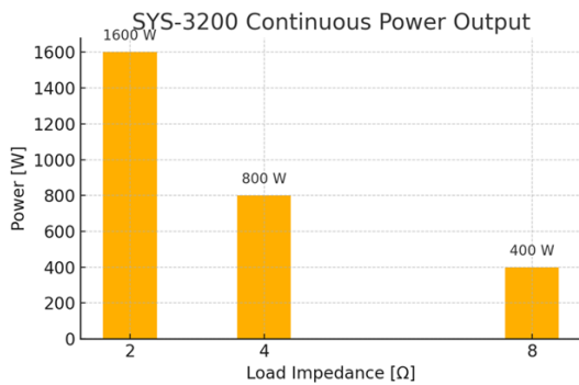
Figura 14: Power Output performance
