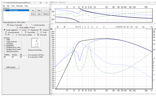
Figura 8: Acoustic curves obtained in the simulation software for the acoustic boxes
