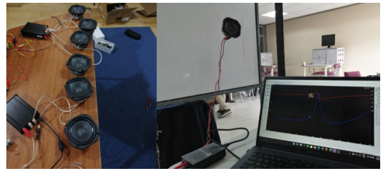
Figura 10: Impedance Response with DATS V3 method
