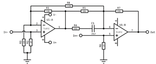
Figura 4: Phase network balanced input
