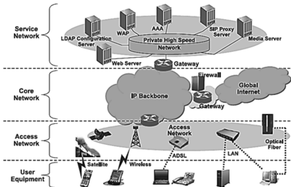
Figure 3. Components of NGN
