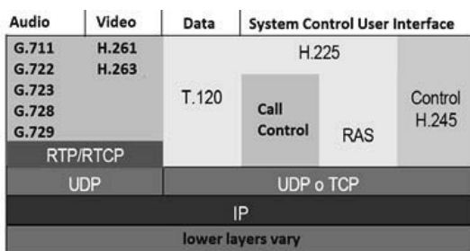
Figure 1. Series-H.323 protocols
