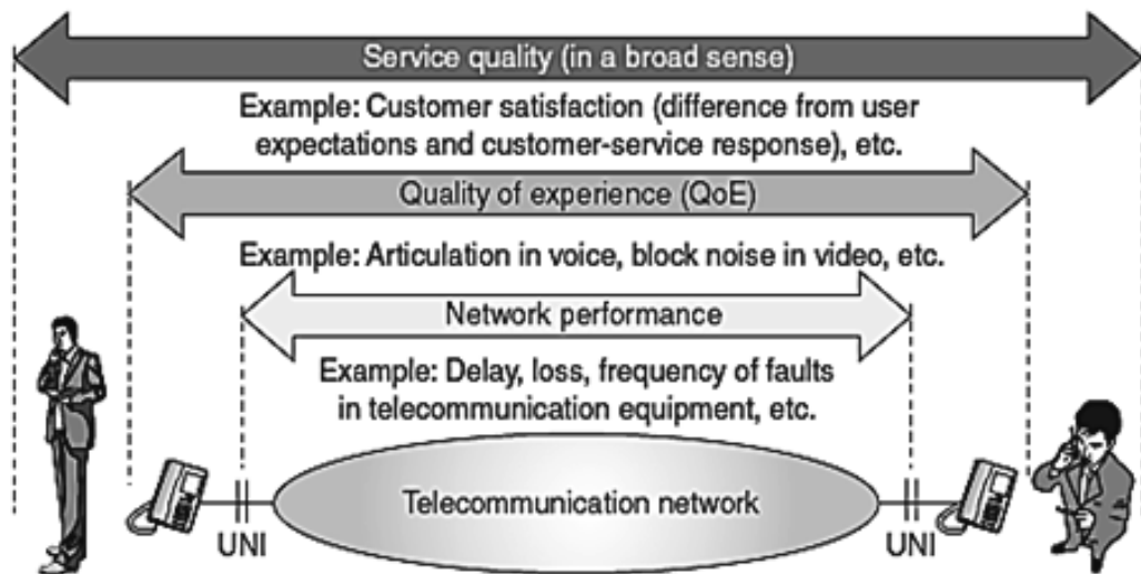
Figure 5. Types of QoS in NGN
