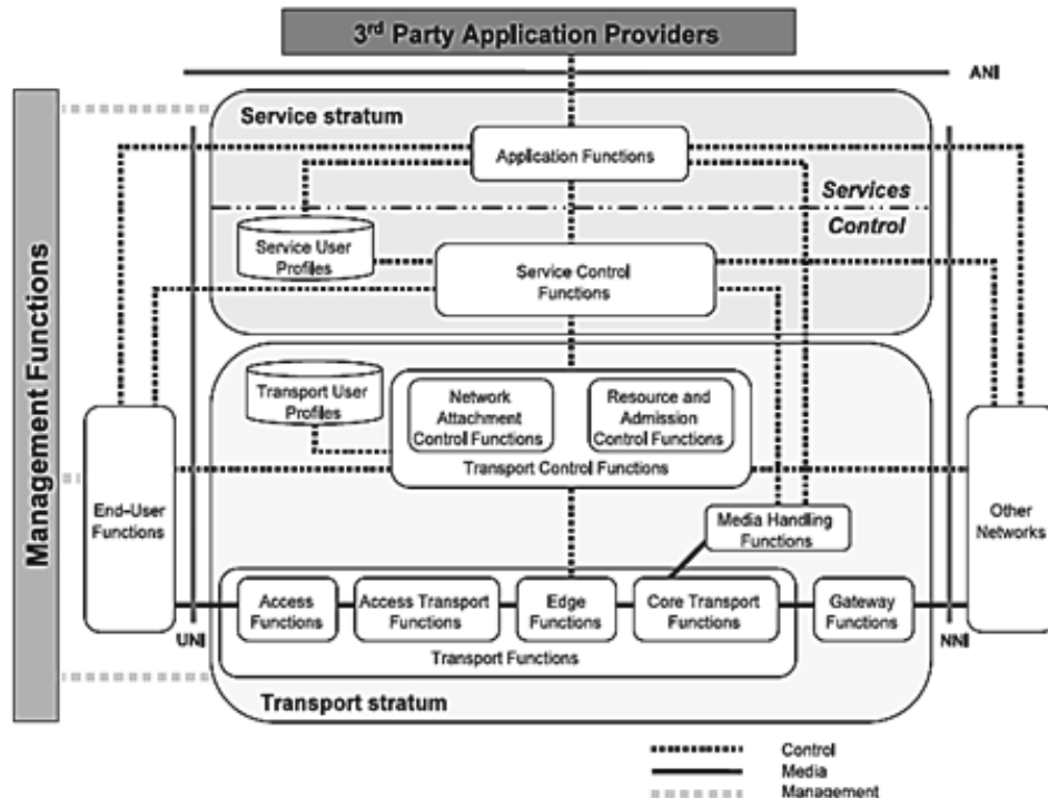
Figure 4. Functional Structure of NGN
