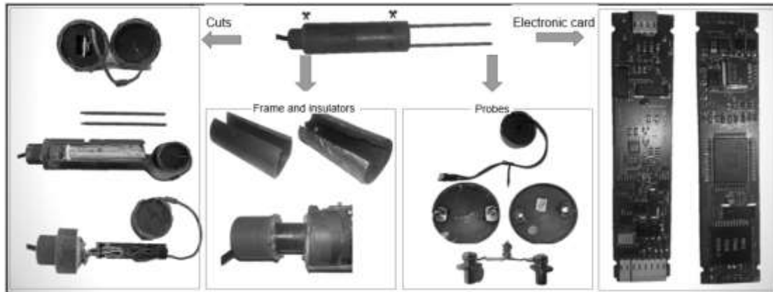
Figure 6. Dissection and classification of TRIME-EZ device elements. Source: own.
