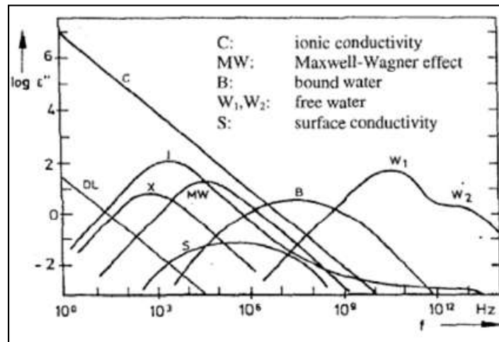
Figure 7. Components in soil polarization related to frequency [12].
