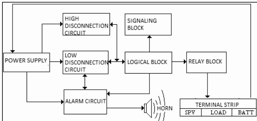
Figure 1. Block diagram of a photovoltaic controller [6].
