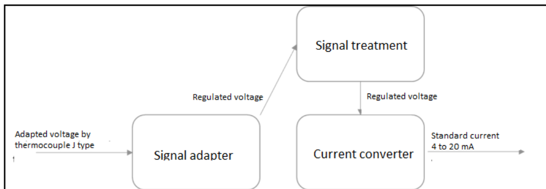
Figure 9. Block diagram for temperature transducer. Source: own.
