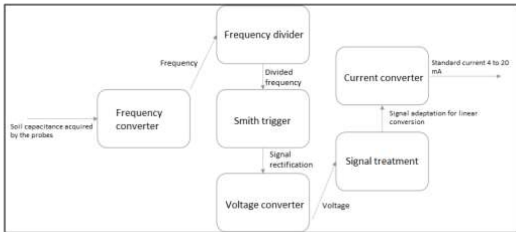
Figure 8. Block diagram for moisture transducer. Source: own.
