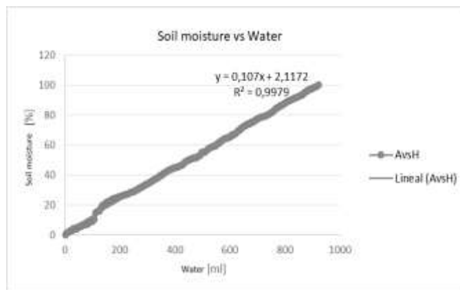
Figure 4. Performance curve of the soil moisture percentage according to the amount of water in the soil. Source: own.
