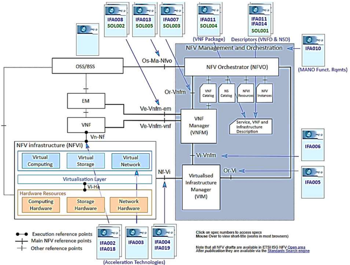
Figure 4. NFV architecture according to ETSI [19].
