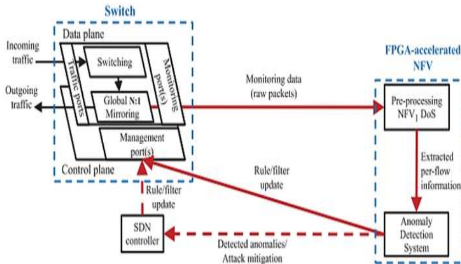
Figure 8. Real-time network security design based on FPGA, [45].
