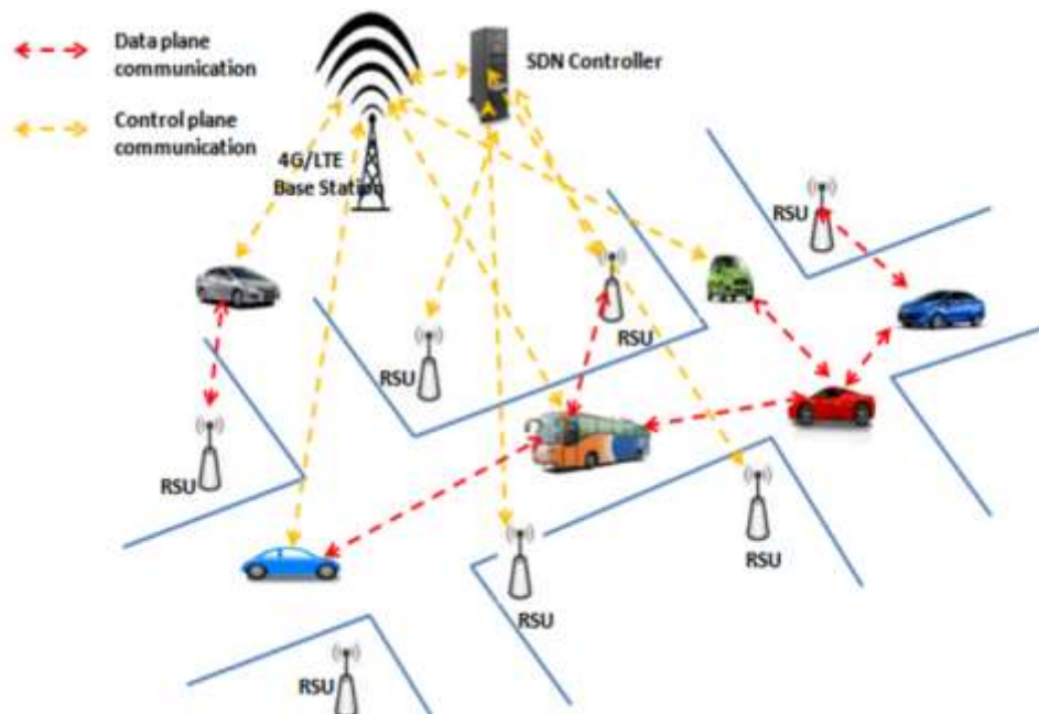
Figure 6. Communication SDN-VANET, [37].
